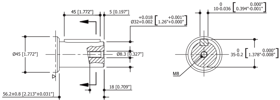
SHAFT B Cylindrical Shaft Ø32 Parallel Key 10 x 8 x 45 METRIC
