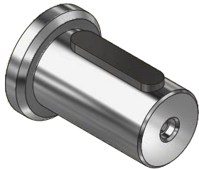
SHAFT B Cylindrical Shaft Ø32 Parallel Key 10 x 8 x 45 METRIC
