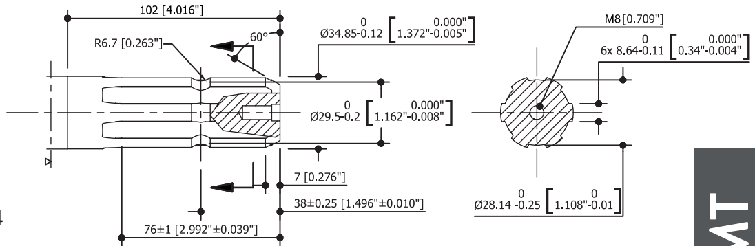
SHAFT SL SPLINED 6-34.85x28.14x8.64
